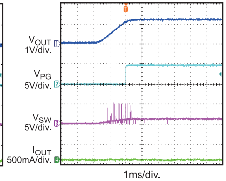
Power Good On without Load
