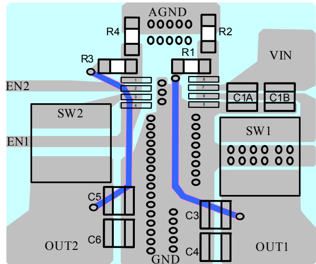
Figure 3: Suggested PCB Layout
