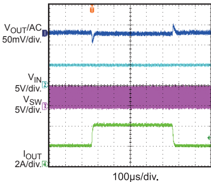
Load Transient Response I_{OUT} = 2A \rightarrow 4A , PWM
