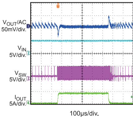
Load Transient Response I_{OUT} = 0A \rightarrow 4A , PFM
