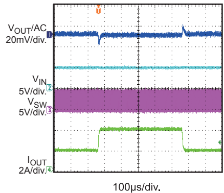
Load Transient Response I_{OUT} = 2A \rightarrow 4A , PFM
