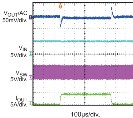
Load Transient Response I_{OUT} = 0A \rightarrow 4A , PWM
