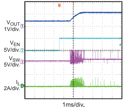
VOUT Prebias Start Up V_{PRE} = 0.5V , I_{OUT} = 0A , PFM
