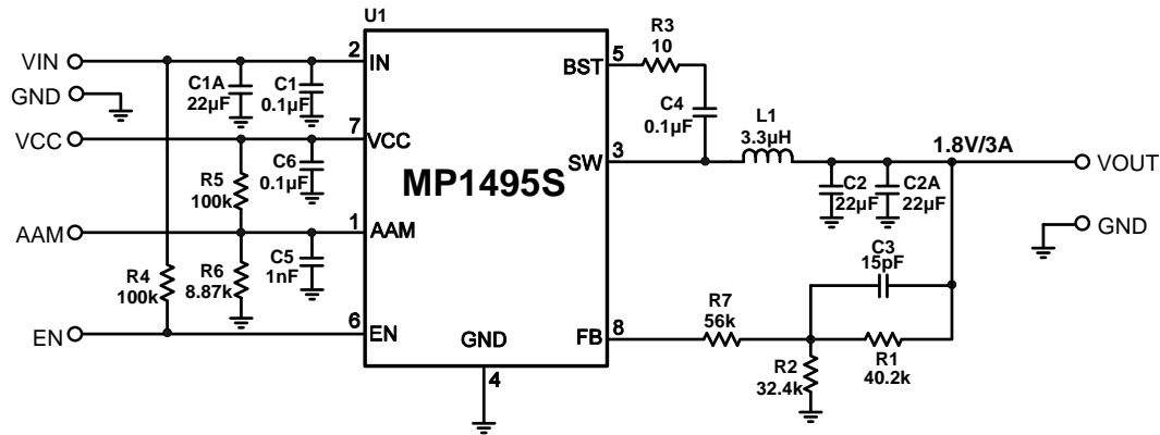
Figure 10: 12V IN , 1.8V/3A Output
