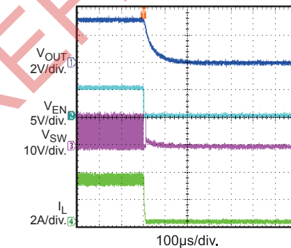
Shutdown through Enable I_{OUT} = 3A
