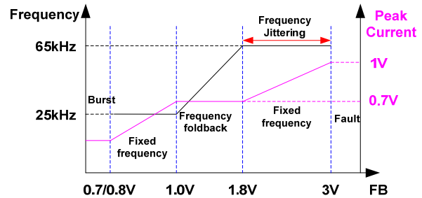
Figure 4: Frequency and Peak Current (V CS ) vs. V FB
