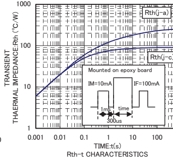
Rth-t CHARACTERISTICS
