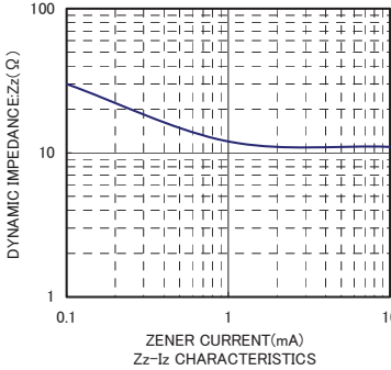
Zz-Iz CHARACTERISTICS
