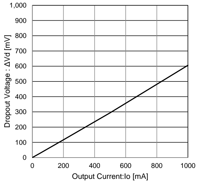
Figure 9. Dropout Voltage (V CC =4.75V) (I o =0mA→1000mA)
