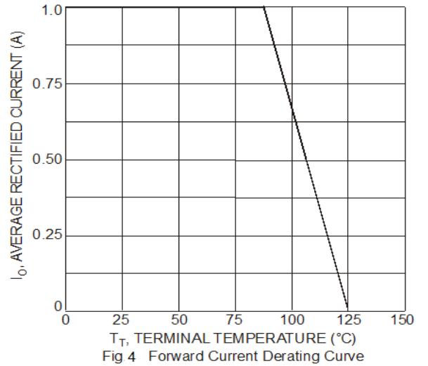
Fig.4 Forward Current Derating Curve
