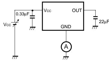
Fig. 4 Measurement circuit for bias current
