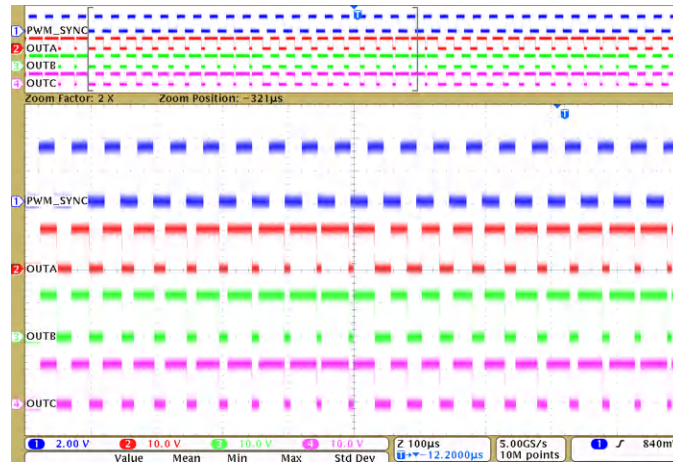
图 10-7. PWM Synchronous Duty Cycle Operation with PWM_SYNC = 2b (10% - 90%) (PWM_SYNC, OUTA, OUTB, OUTC)
