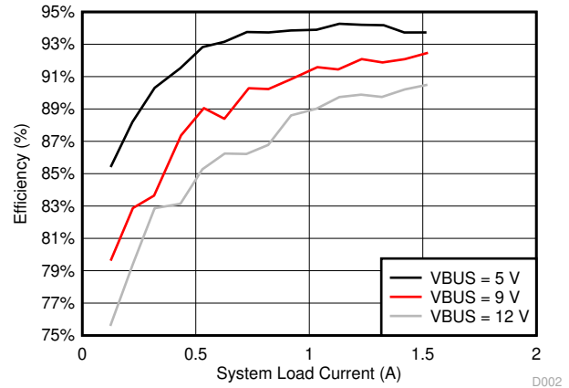
图 8-2. System Light Load Efficiency vs System Light Load Current
