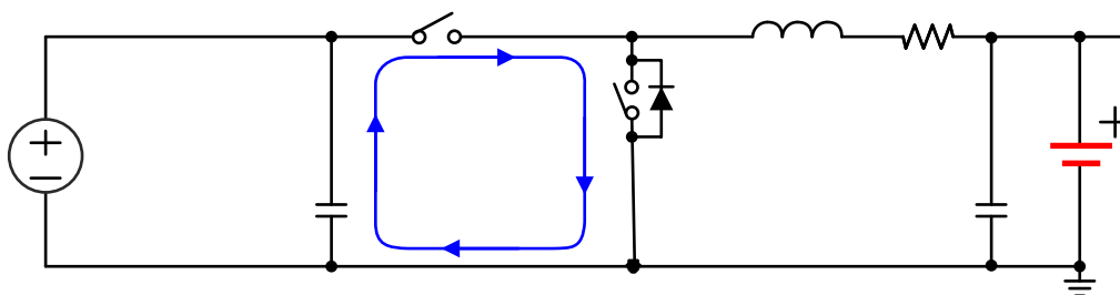
图 12-1. High Frequency Current Path
