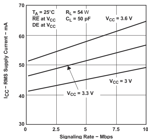
图 7-2. HVD11 RMS Supply Current vs Signaling Rate
