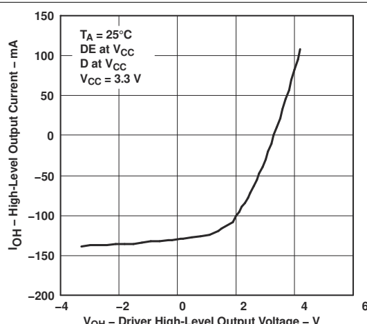
图 7-6. High-Level Output Current vs Driver High-Level Output Voltage
