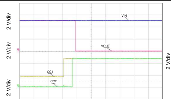
图 24. Hot-Plug to Short
