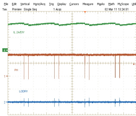
CH1: PHASE, 10V/div, CH2: LODRV, 5V/div, CH3: inductor current, 2A/div, 4us/div
