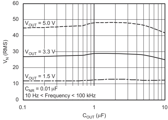
Legacy silicon 图 5-31. RMS Noise Voltage vs C_{OUT}
