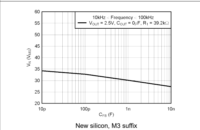
图 7-8. TPS73201 RMS Noise Voltage vs C_FB
