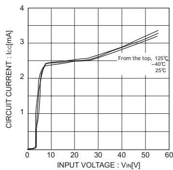
Fig.8 Circuit current (BD9001F)
