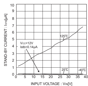
Fig.3 Standby current (BD9781HFP)
