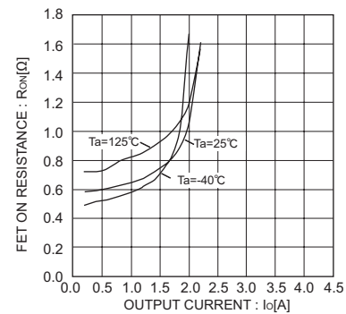
Fig.9 ON resistance V_{IN}=5V (BD9781HFP)
