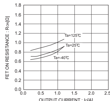
Fig.12 ON resistance V_{IN}=5V (BD9778F/HFP)
