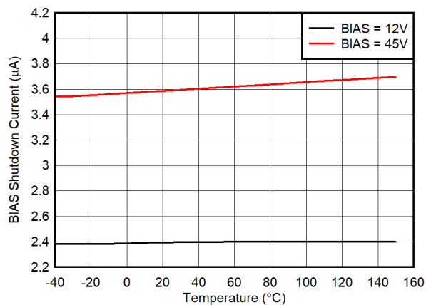
图 8-2. BIAS Shutdown Current vs Temperature
