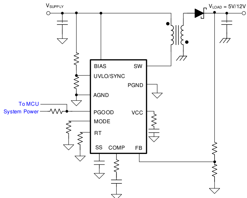
图 10-12. Typical Non-Isolated Flyback
