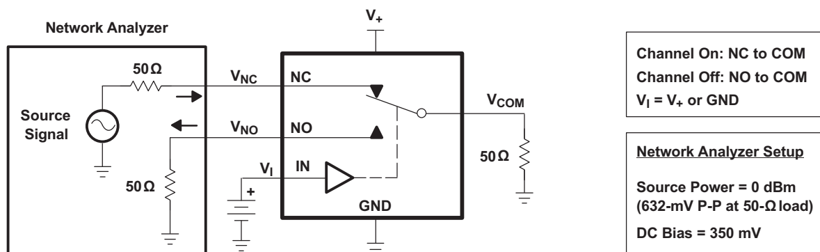
Figure 22. Crosstalk (X TALK )
