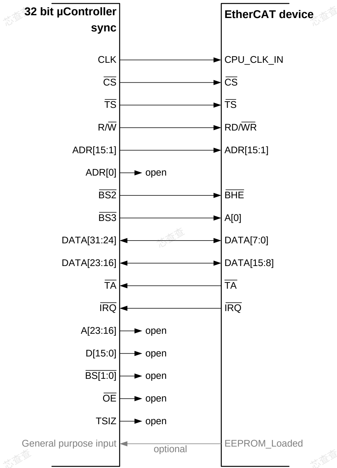
Figure 39: Synchronous 32 bit \mu Controller connection using Byte Select
