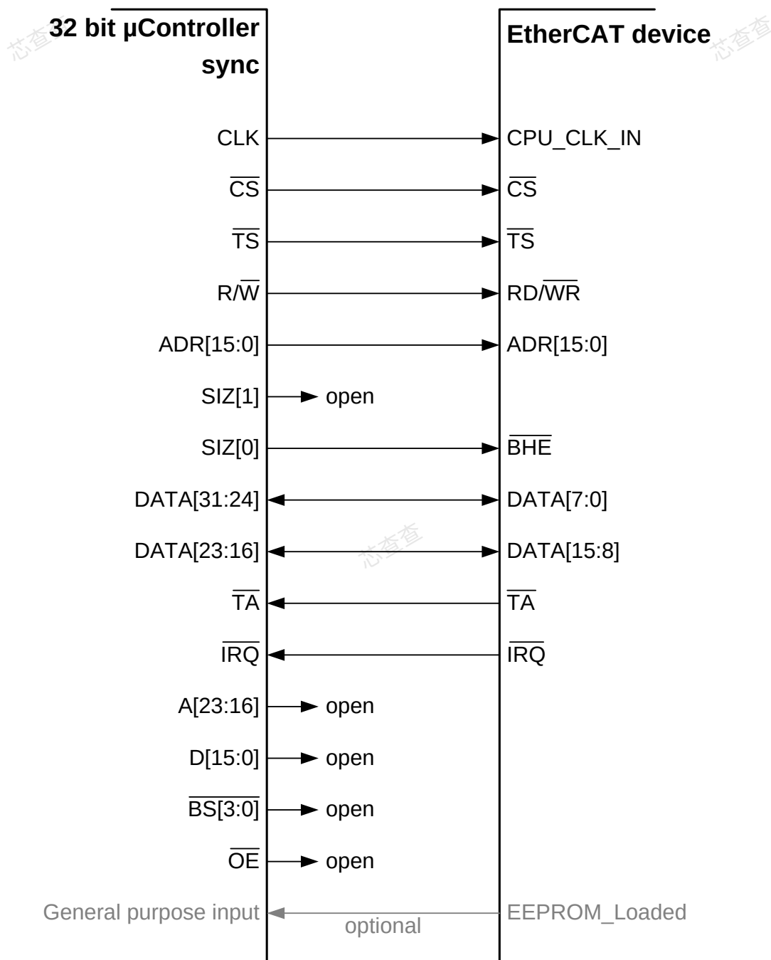
Figure 41: Synchronous 32 bit \mu Controller connection using Transfer Size
