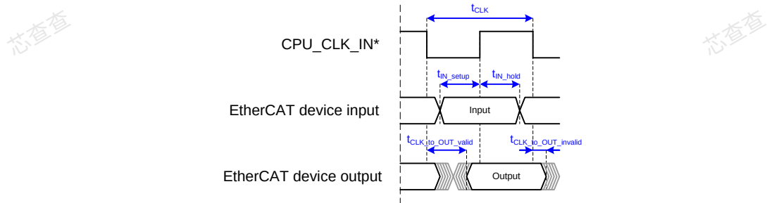
Figure 42: Basic synchronous \mu Controller interface timing (*refer to timing diagram for relevant CPU_CLK_IN edges)
