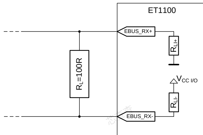
Figure 12: LVDS termination
