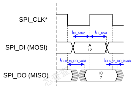
Figure 27: Basic SPI_DI/SPI_DO timing (*refer to timing diagram for relevant edges of SPI_CLK)
