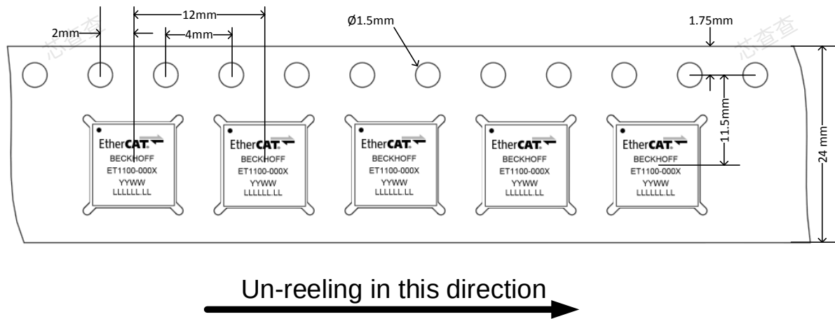
Figure 57: ET100 Tape Information
