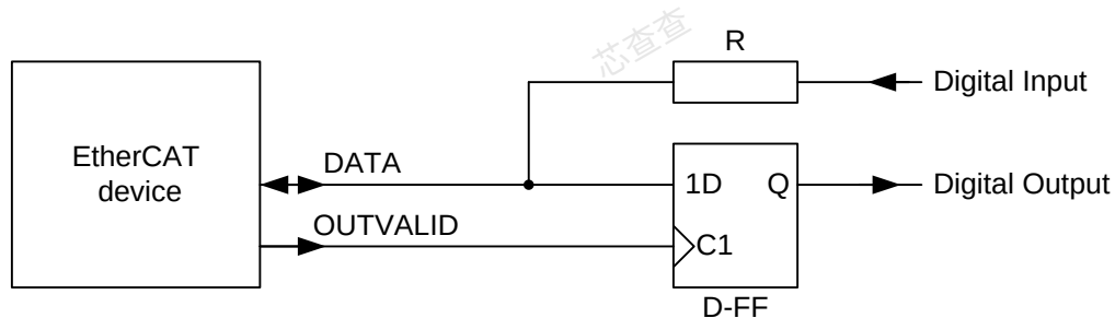
Figure 21: Bidirectional mode: Input/Output connection (R=4.7 kΩ recommended)
