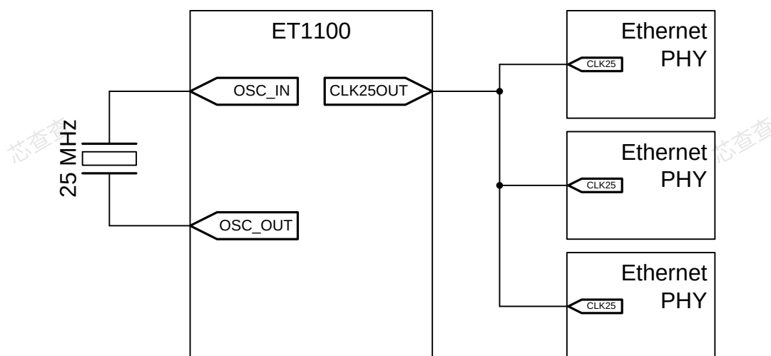
Figure 5: Quartz crystal Clock source for ET1100 and Ethernet PHYs
