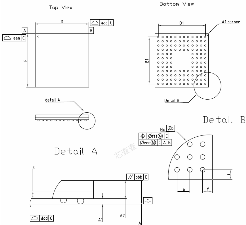
Figure 54: Package Outline
