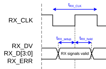
Figure 17: MII timing RX signals
