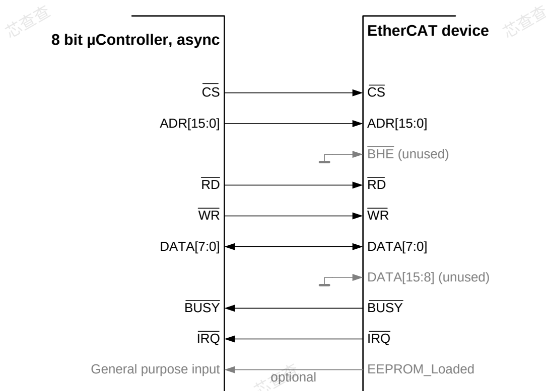
Figure 34: Connection with 8 bit \mu Controllers (BHE and DATA[15:8] should not be left open)
