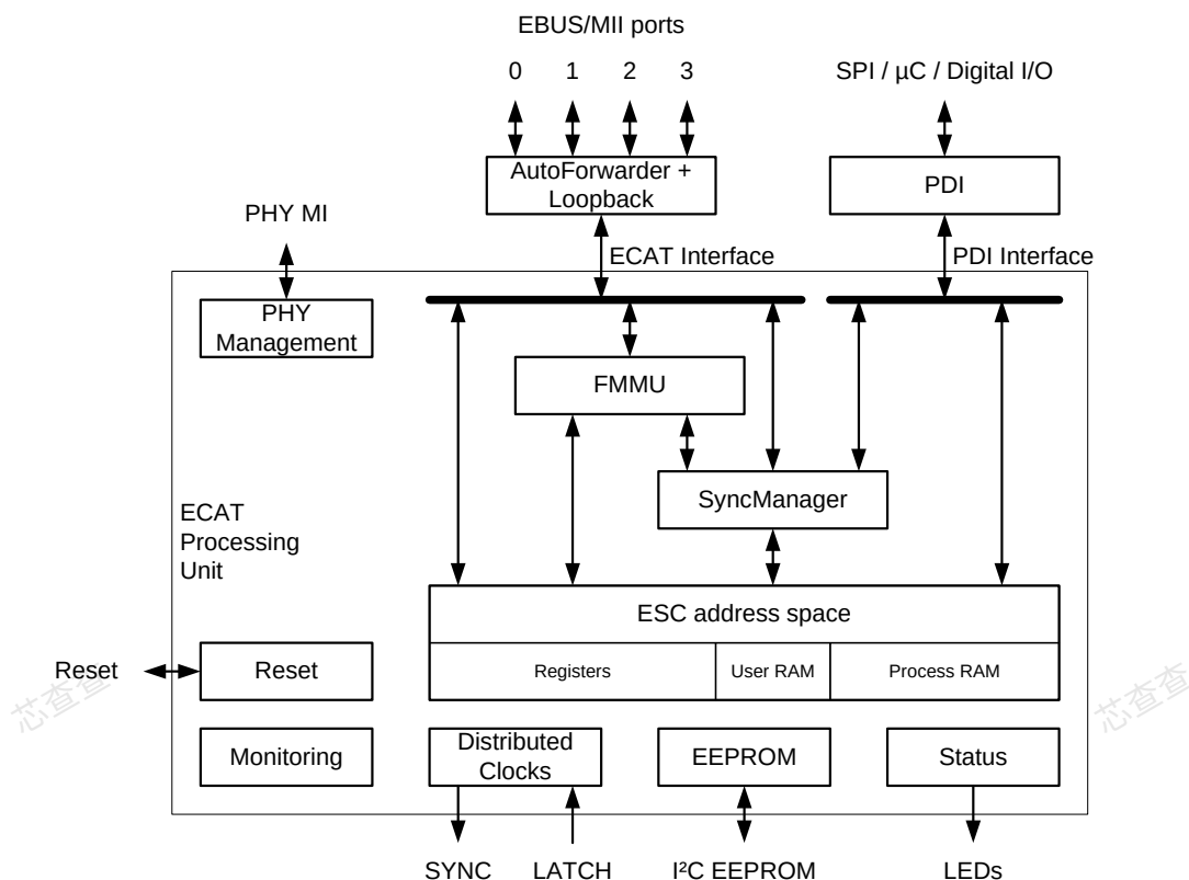
Figure 1: ET1100 Block Diagram
