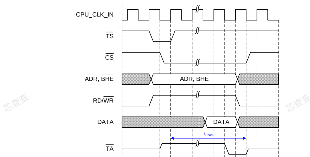
Figure 47: Read access (CS half a clock period after TS, CS and TA on falling edge)
