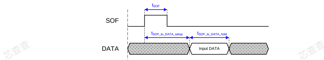
Figure 22: Digital Input: Input data sampled at SOF, I/O can be read in the same frame
