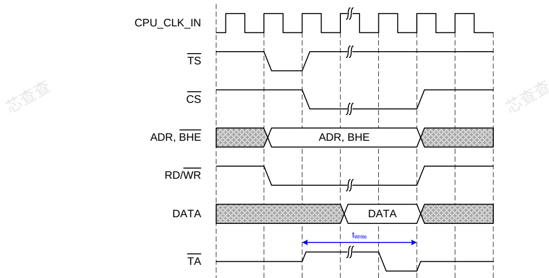
Figure 45: Write access (CS after TS, Write DATA after CS, CS and TA on rising edge)
