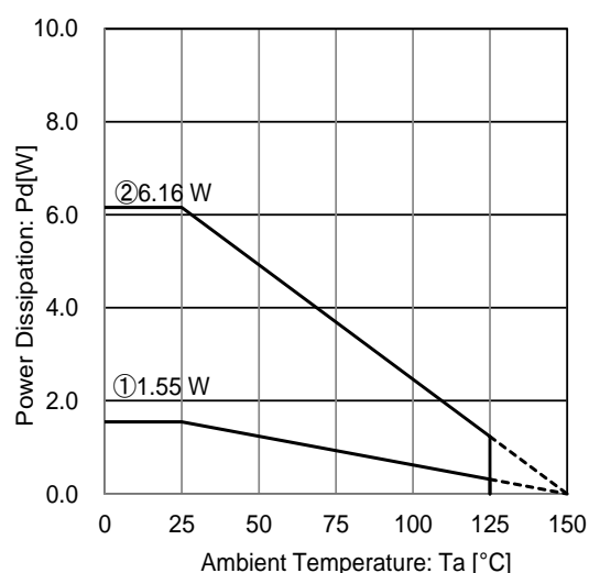
Figure 22. TO263-5 Package Data
