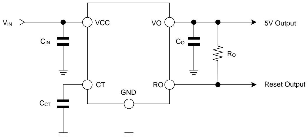
Figure 2. Application Circuit
