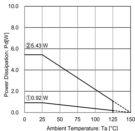
Figure 23. TO252-J5 Package Data
