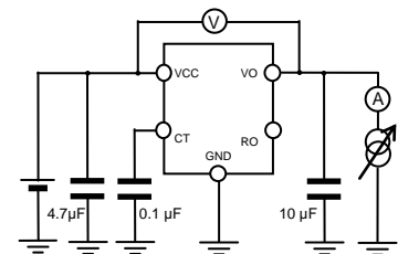
Measurement Circuit for Figure.13
