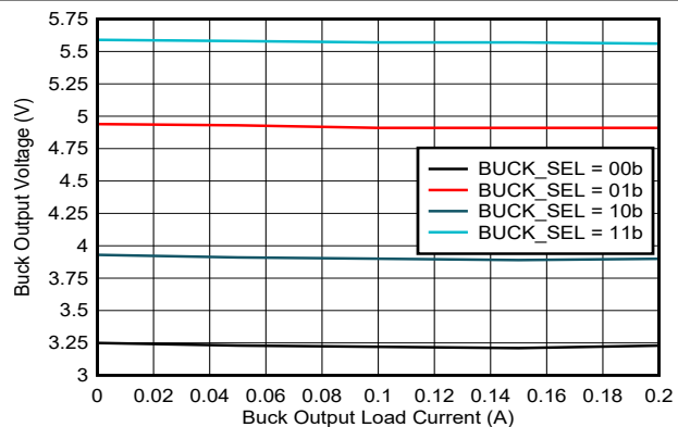
图 7-5. Buck regulator output voltage over load current
