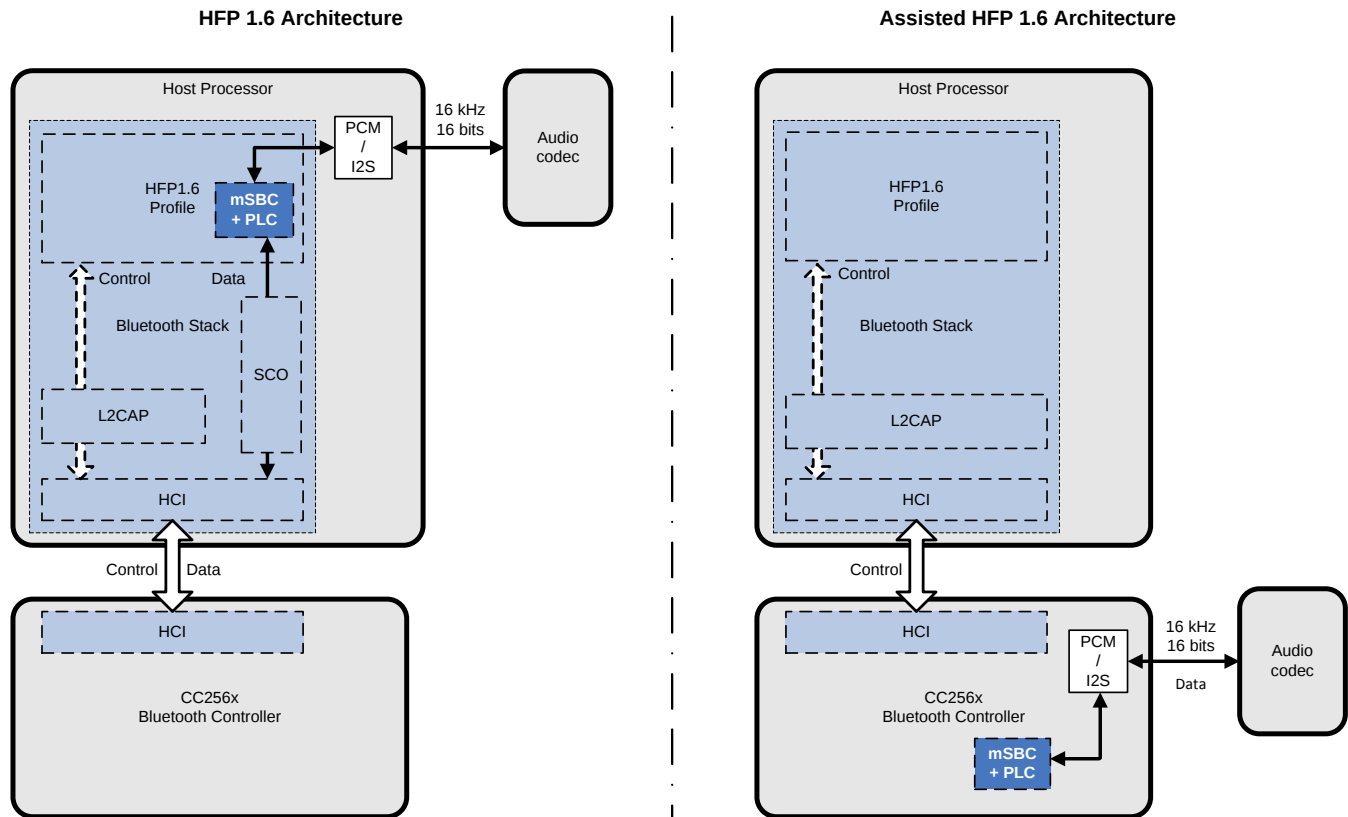
Figure 6-15. HFP 1.6 Architecture Versus Assisted HFP 1.6 Architecture
