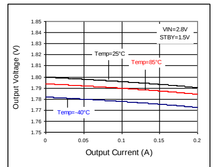
Fig 8. Load Regulation
