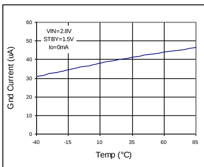
Fig 12. IGND - Temp
