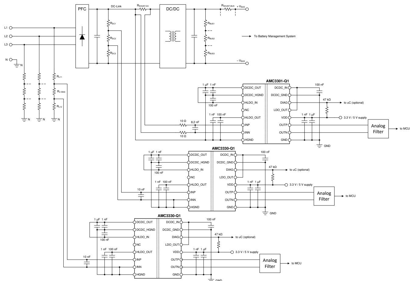
图 7-1. The AMC3330-Q1 in an OBC Application
