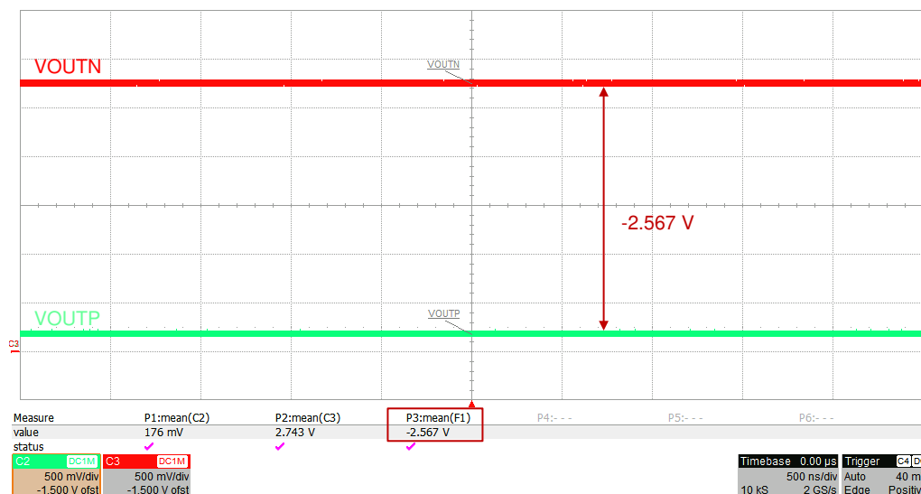
图 6-5. Typical Fail-Safe Output of the AMC3330-Q1
