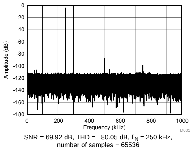
Figure 3. Typical FFT
