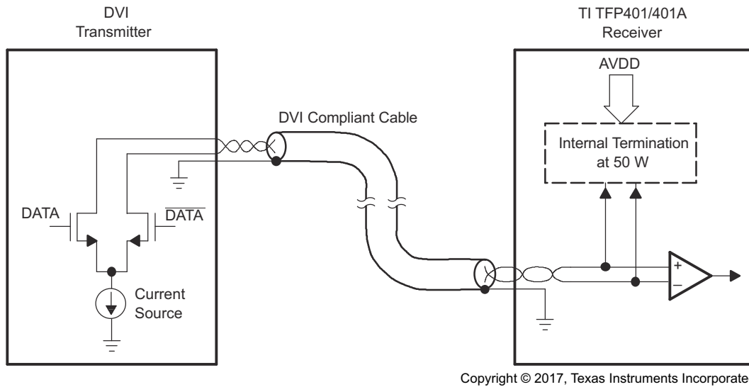
图 7-1. TMDS Differential Input and Transmitter Connection
