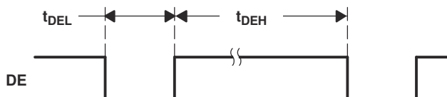
图 6-13. Minimum DE Low and Maximum DE High
