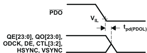
图 6-7. Delay From PDO Low to Hi-Z Outputs
