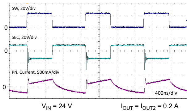
图 8-12. Typical Switching Waveforms
