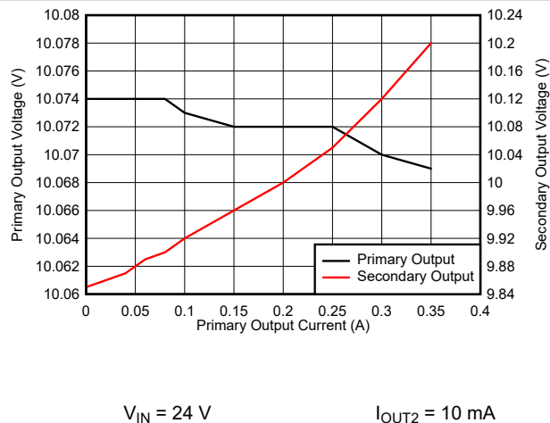
图 8-3. Load Regulation vs Primary Load Current
