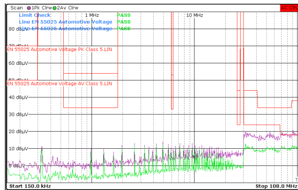
图 8-37. LM5169PDDAR Conducted EMI (Positive Rail)
