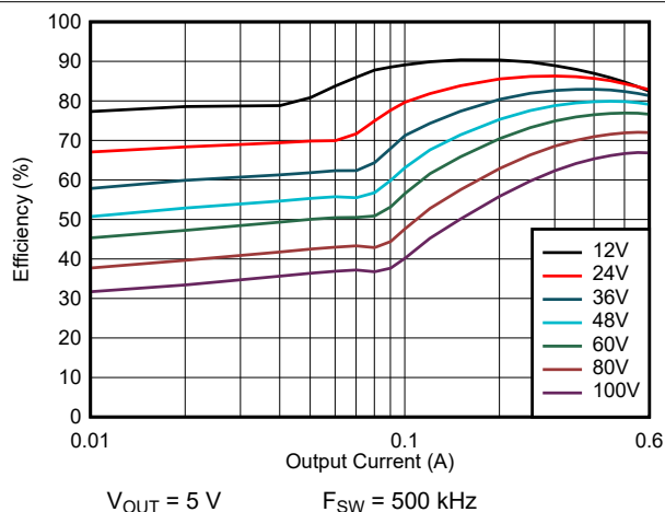
图 8-15. Efficiency: V_{OUT} = 5\text{ V}
