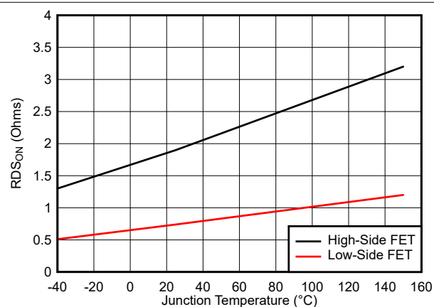
图 6-6. MOSFETs On-State Resistance Versus Temperature
