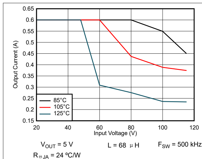
图 8-35. Maximum Output Current: V_{OUT} = 5\text{ V}
