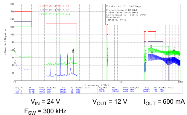
图 8-38. LM5169PDDAR Conducted EMI (Negative Rail)
