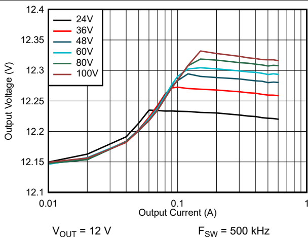
图 8-19. Line and Load Regulation: V_{OUT} = 12\text{ V}
