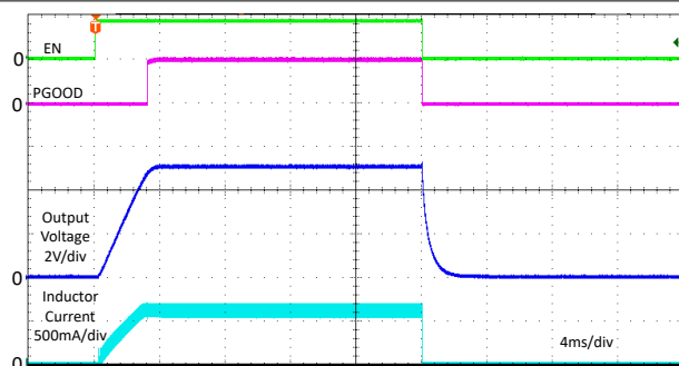
图 8-27. Typical Switching Waveforms
