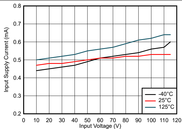
图 6-3. Active Mode Supply Current Versus Input Voltage (FPWM, non-switching)
