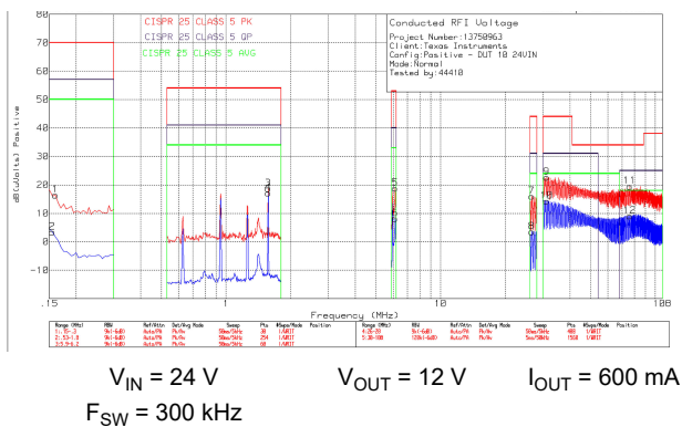
图 8-37. LM5169PDDAR Conducted EMI (Positive Rail)
