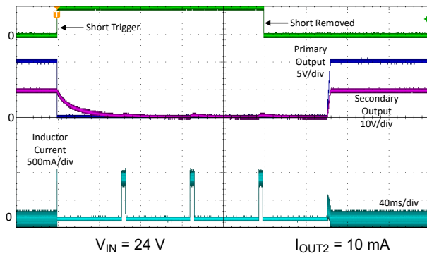
图 8-10. Short Circuit on Primary Output
