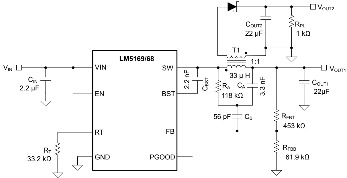
图 8-1. Example Fly-Buck™ Converter Application Circuit
