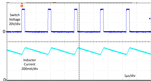
图 8-27. Typical Switching Waveforms
