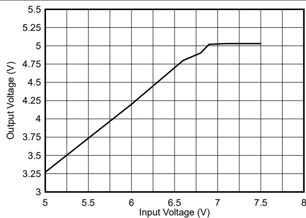
图 8-31. Drop-Out Response
