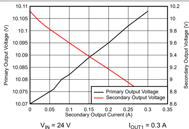
图 8-4. Load Regulation vs Secondary Load Current
