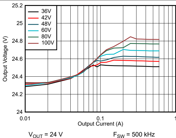
图 8-20. Line and Load Regulation: V_{OUT} = 24\text{ V}
