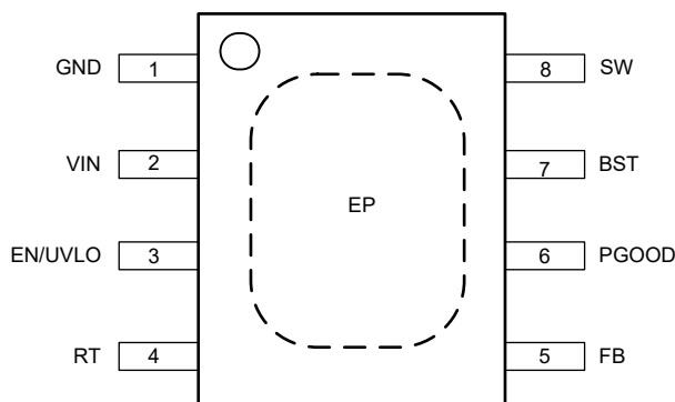
图 5-1. 8-Pin SO PowerPAD™ Integrated Circuit Package (Top View)
