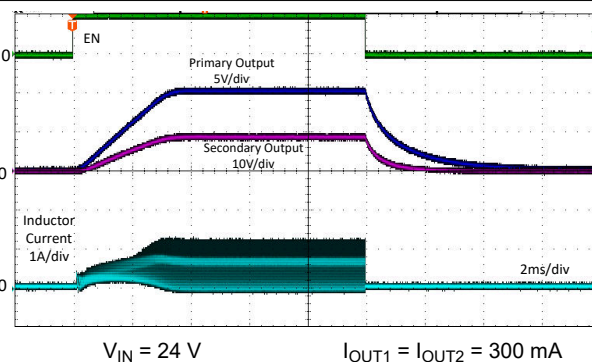
图 8-7. Full Load Start-Up from EN
