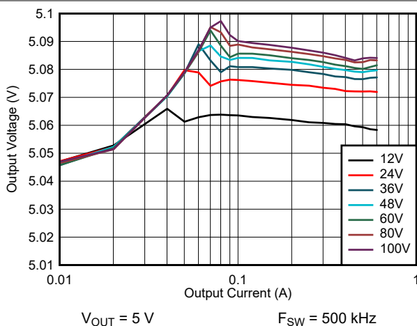
图 8-18. Line and Load Regulation: V_{OUT} = 5\text{ V}
