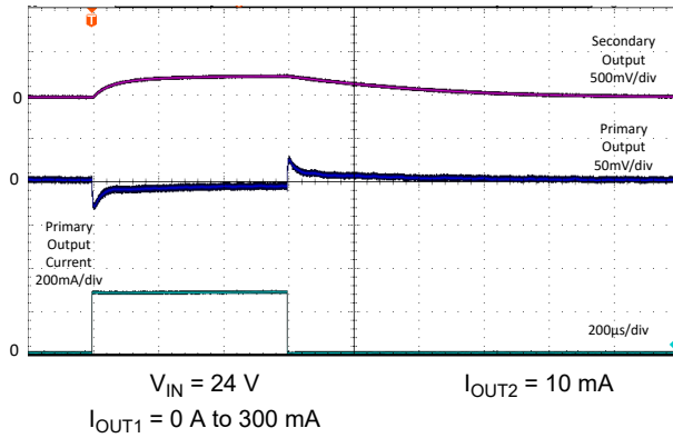
图 8-8. Load Transient on Primary Output
