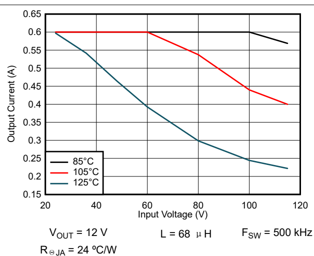
图 8-36. Maximum Output Current: V_{OUT} = 12\text{ V}
