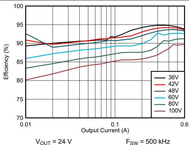
图 8-17. Efficiency: V_{OUT} = 24\text{ V}
