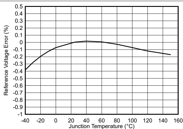
图 6-5. Feedback Comparator Threshold Versus Temperature
