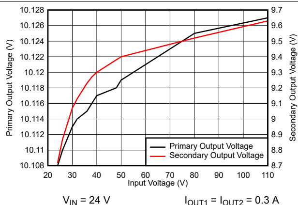
图 8-5. Line Regulation
