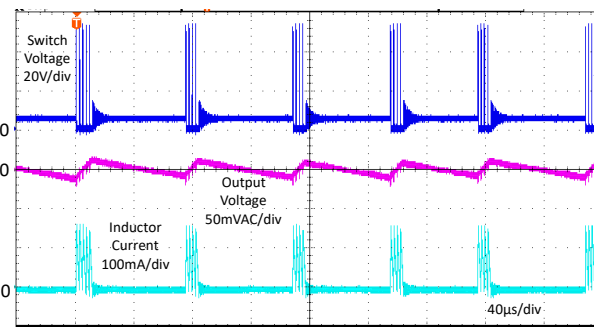
图 8-28. Typical Switching Waveforms
