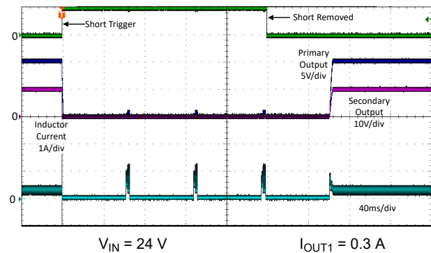
图 8-11. Short Circuit on Secondary Output
