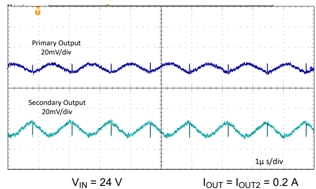
图 8-13. Typical Output Ripple
