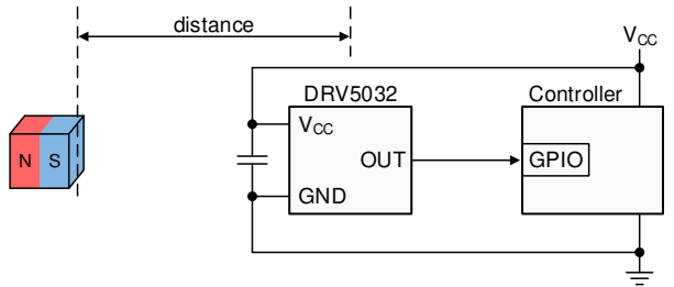
Copyright © 2017, Texas Instruments Incorporated 典型电路原理图
