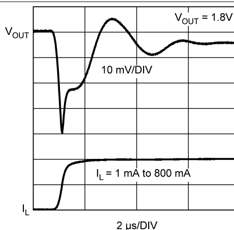
Figure 30. Load Transient Response
