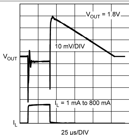
Figure 29. Load Transient Response
