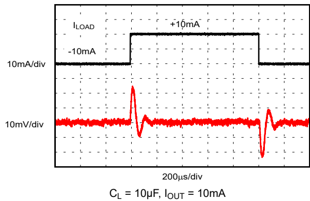
Figure 6-20. Load Transient
