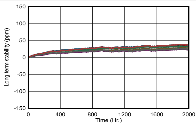
Figure 6-50. Long-Term Stability (First 2000 Hours)
