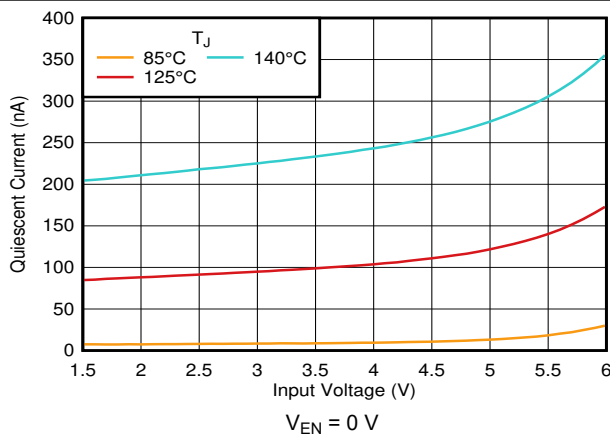
图 6-11. I_{SHDN} vs V_{IN} and Temperature
