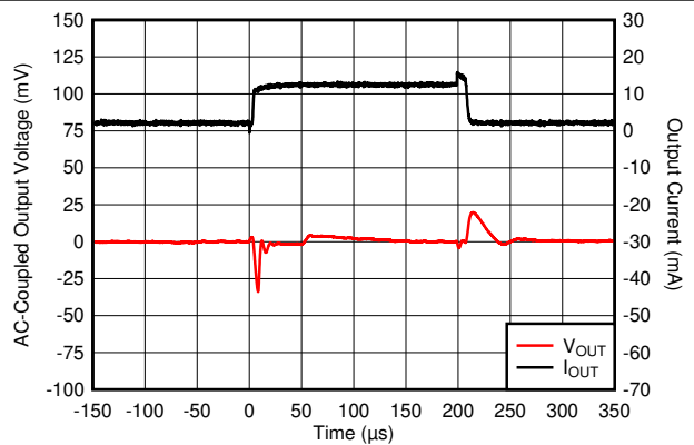
图 6-12. I_{OUT} Transient From 1 mA to 10 mA
