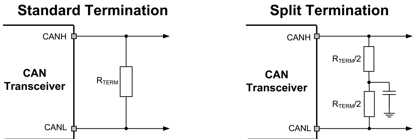
Figure 31. CAN Termination
