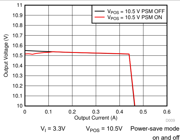
图 8-6. Boost Converter ( V_{POS} ) Output Voltage vs Output Current
