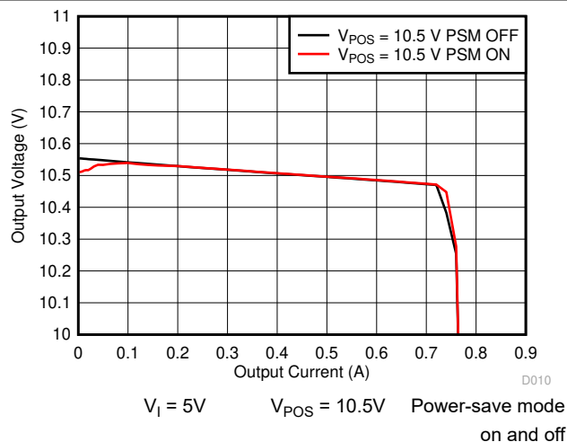
图 8-7. Boost Converter ( V_{POS} ) Output Voltage vs Output Current
