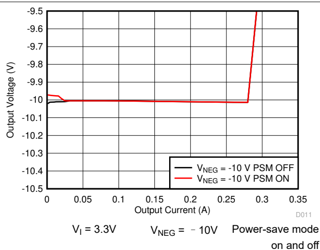
图 8-8. Inverting Converter ( V_{NEG} ) Output Voltage vs Output Current
