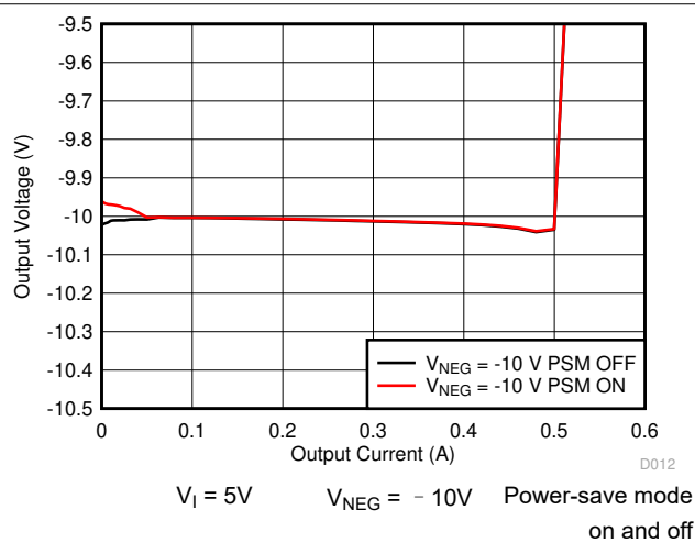
图 8-9. Inverting Converter ( V_{NEG} ) Output Voltage vs Output Current
