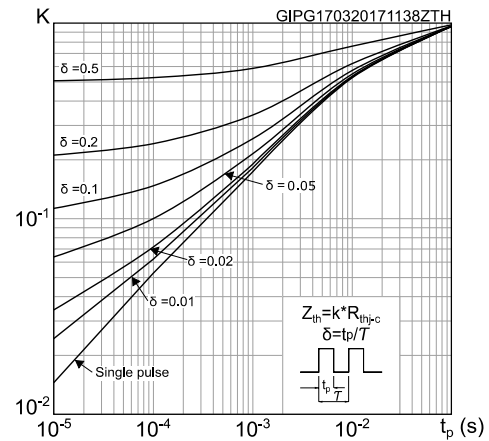
Figure 3: Thermal impedance
