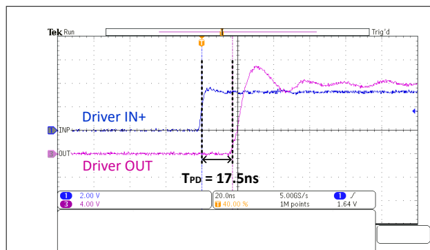
图 8-3. UCC27614 Rising (Turn-On) Propagation Delay
