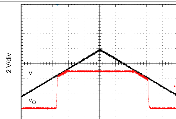
Figure 58. Low-Dropout Operation
