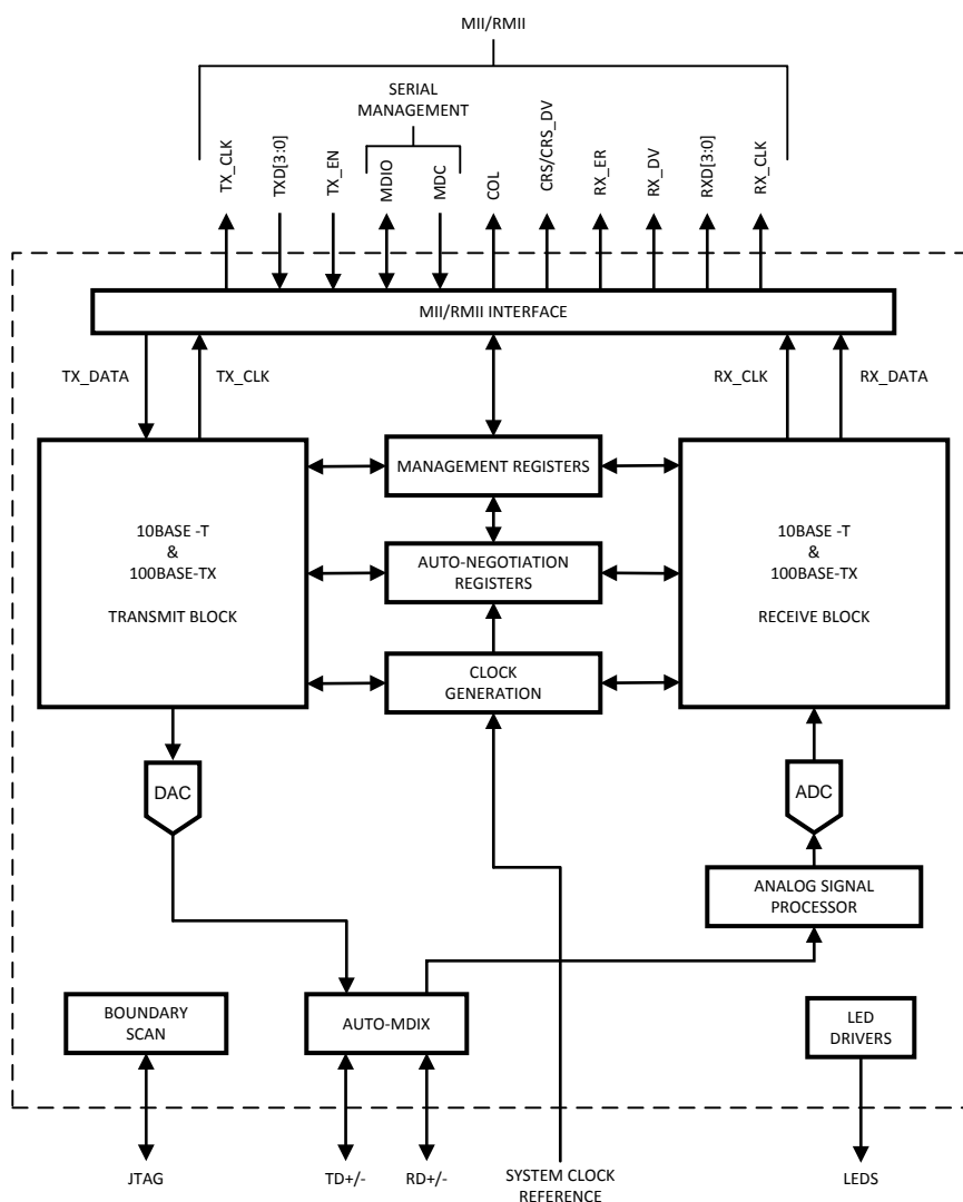
Figure 2-1. DP83620 Functional Block Diagram
