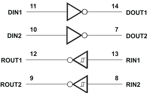
图 6-1. Logic Diagram (Positive Logic)
