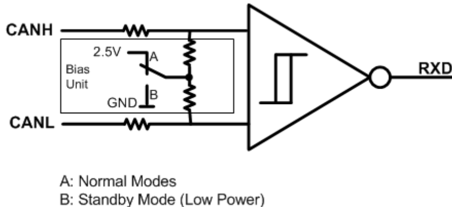
图 9-3. Bias Unit (Recessive Common Mode Bias) and Receiver
