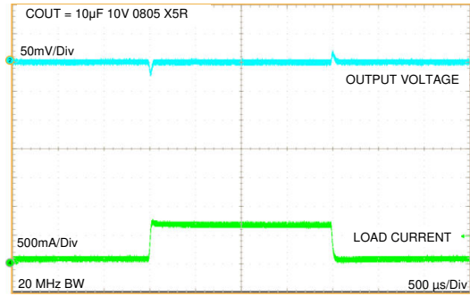
图 8-5. Load Transient V_{OUT} = 1.2\text{ V}
