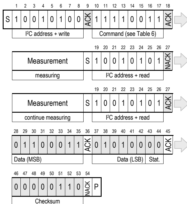
Figure 13 No Hold master communication sequence – grey blocks are controlled by STS21. If measurement is not completed upon "read" command, sensor does not provide ACK on bit 27 (more of these iterations are possible). If bit 45 is changed to NACK followed by Stop condition (P) checksum transmission is omitted.
