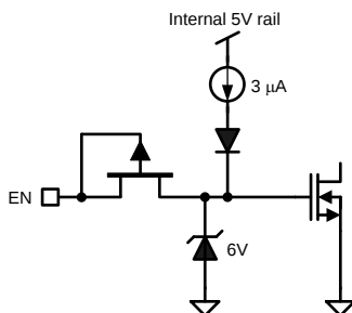
Figure 29. Enable Circuit
