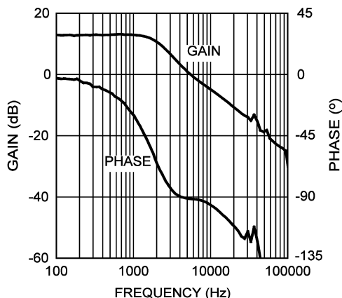
Figure 36. Modulator Gain and Phase
