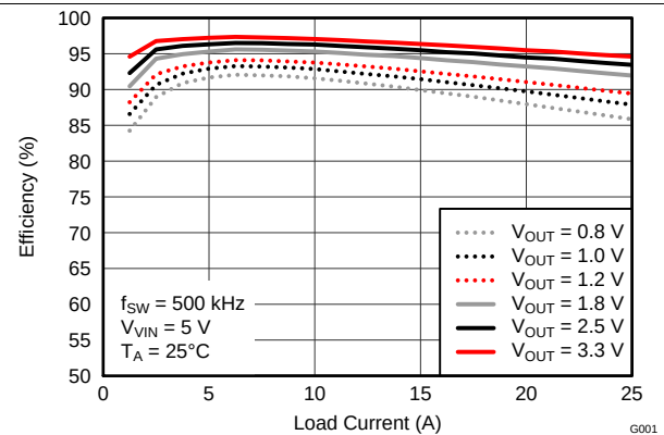
图 16. Efficiency vs. Load Current (VIN = 5 V)
