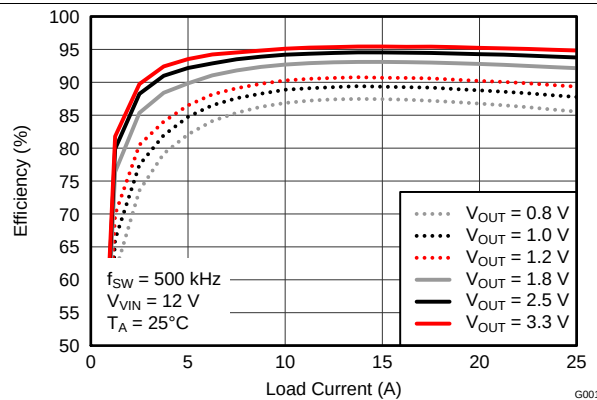
图 15. Efficiency vs. Load Current (VIN = 12 V)
