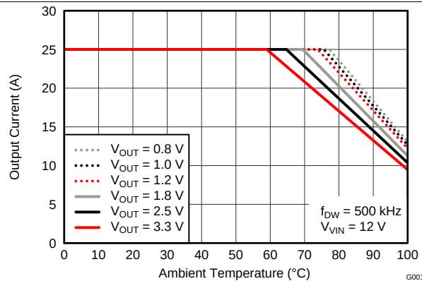
图 17. Output Current vs. Ambient Temperature (VIN = 12 V)
