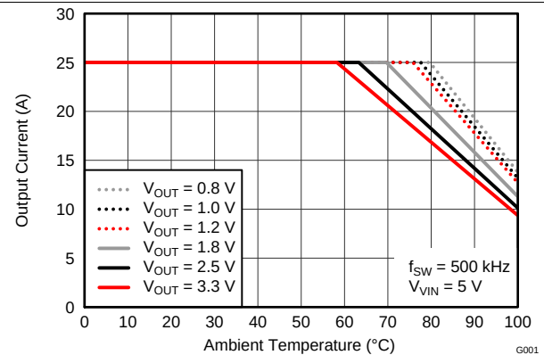
图 18. Output Current vs. Ambient Temperature (VIN = 5 V)
