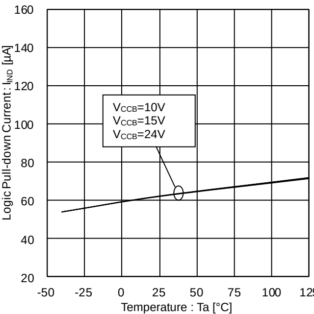
Figure 19. Logic Pull-down Current vs Temperature
