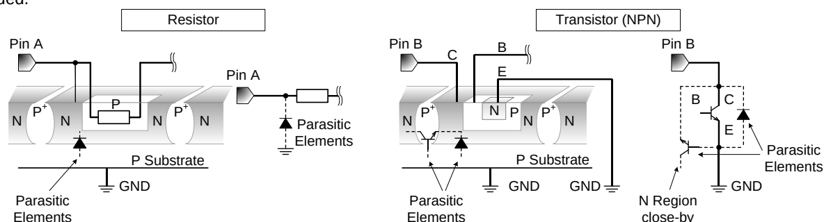
Figure 38. Example of IC structure
