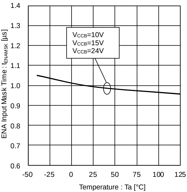
Figure 21. ENA Input Mask Time vs Temperature
