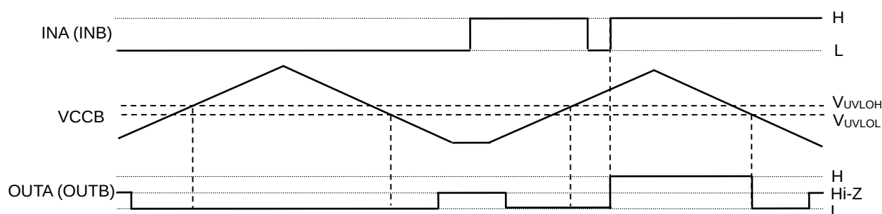
Figure 7. Low-side UVLO Function Operation Timing Chart
