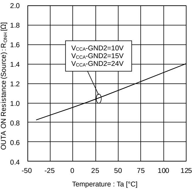
Figure 22. OUTA ON Resistance (Source) vs Temperature
