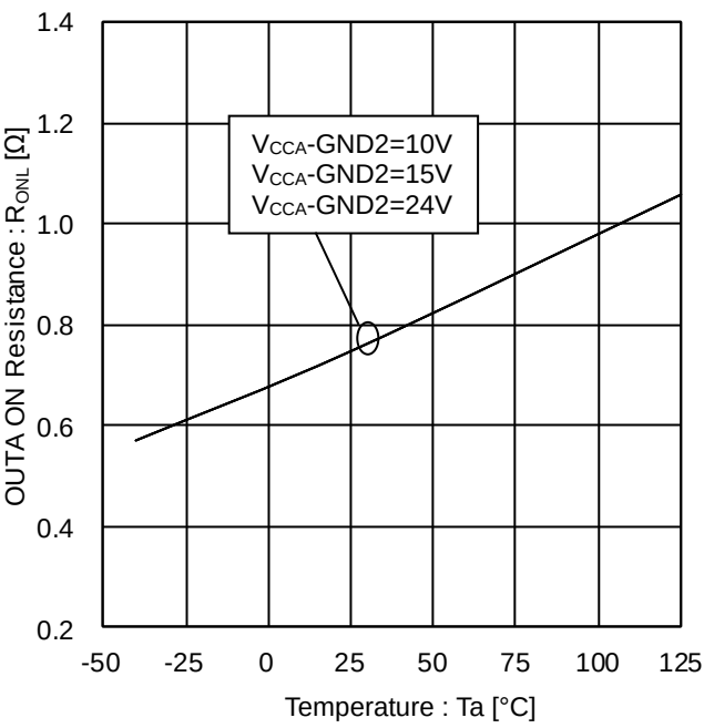
Figure 23. OUTA ON Resistance (Sink) vs Temperature
