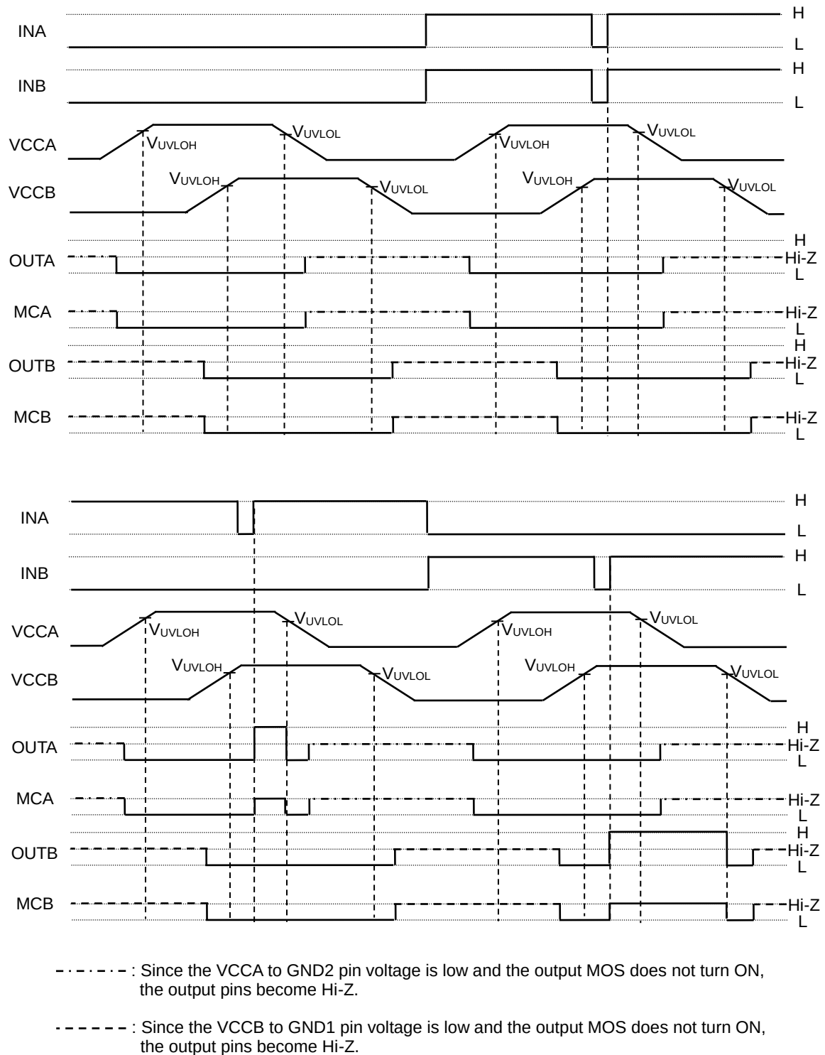
Figure 8. Power Supply Startup/Shutdown Sequence
