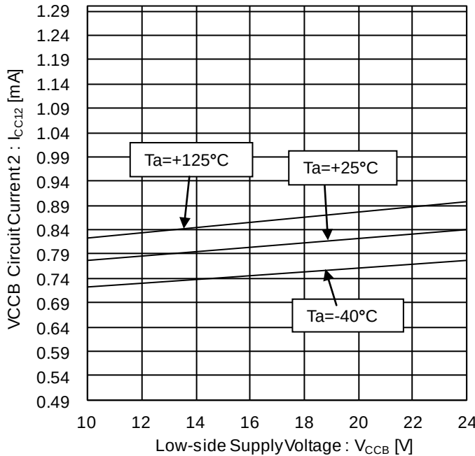
Figure 11. VCCB Circuit Current 2 vs Low-side Supply Voltage (OUTB=H)
