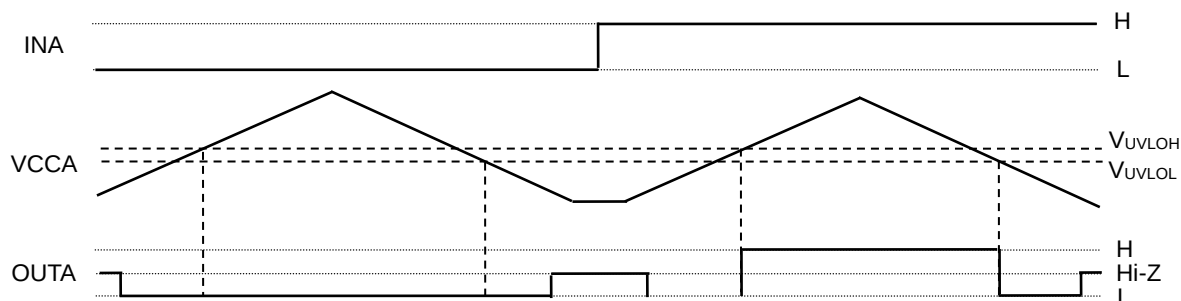
Figure 6. High-side UVLO Function Operation Timing Chart
