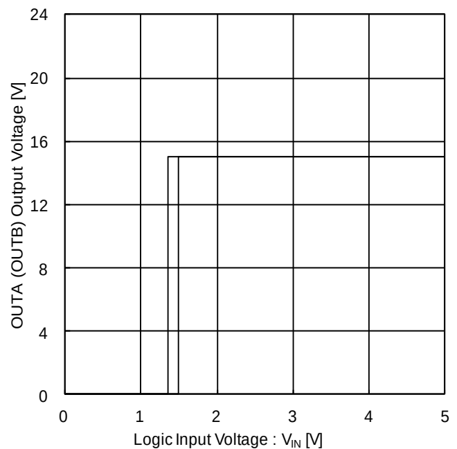
Figure 17. OUTA ( OUTB ) Output Voltage vs Logic Input Voltage ( V_{CCB}=15\text{V} , V_{CCA}=15\text{V} , T_a=+25^\circ\text{C} )
