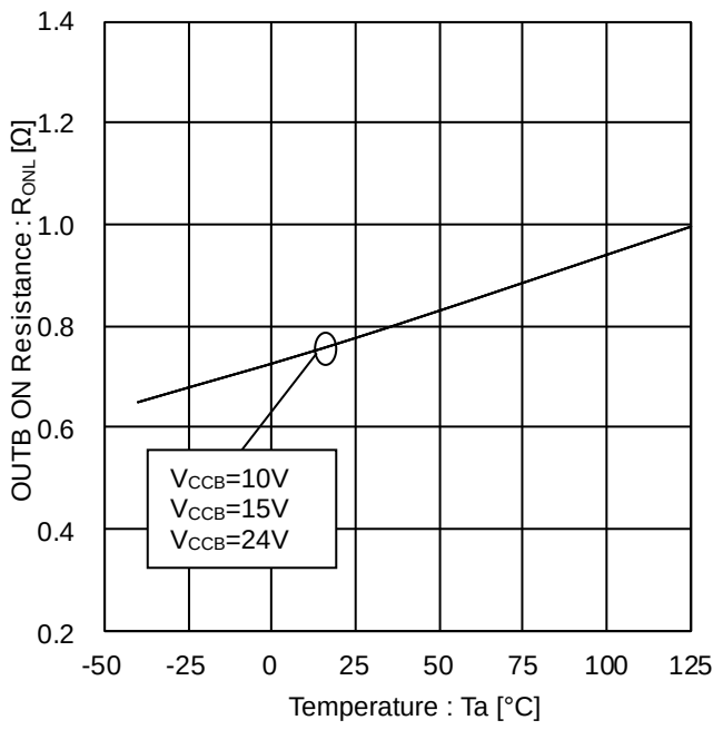
Figure 25. OUTB ON Resistance (Sink) vs Temperature
