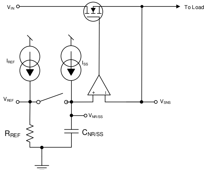
图 7-1. Simplified Regulation Circuit
