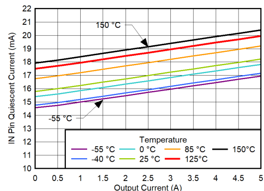
图 6-152. IN Pin Quiescent Current vs I_{OUT} for V_{OUT} = 5.2\text{ V} , CP Enabled
