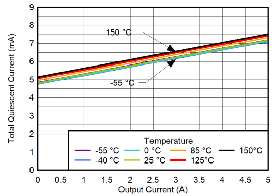
图 6-144. Total Quiescent Current vs I_{OUT} for V_{OUT} = 5.2 \text{ V} , V_{BIAS} = 11 \text{ V} , CP Disabled
