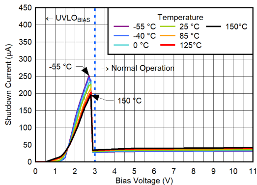
图 6-197. IN Pin Shutdown Current vs V_{BIAS} for V_{IN} = 0.7\text{ V} , V_{OUT} = 0.5\text{ V} , CP Enabled
