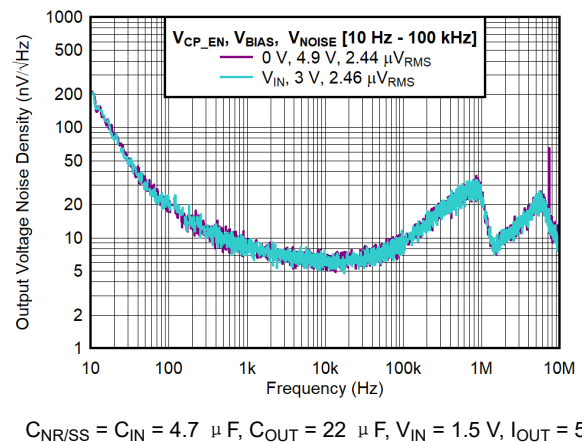
图 6-22. Output Voltage Noise Density vs Frequency and V_{CP\_EN} for V_{OUT} = 1.2\text{ V}
