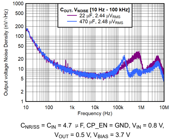
图 6-19. Output Voltage Noise Density vs Frequency and C_{OUT}
