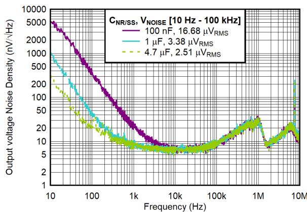
图 8-6. Output Voltage Noise Density vs C_{NR/SS} With Charge Pump Enabled
