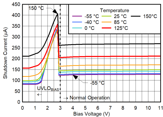
图 6-205. BIAS Pin Shutdown Current vs V_{BIAS} for V_{IN} = 6\text{ V} , V_{OUT(nom)} = 0.5\text{ V} , CP Disabled
