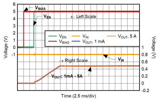
图 8-43. Start-Up Rail Sequence
