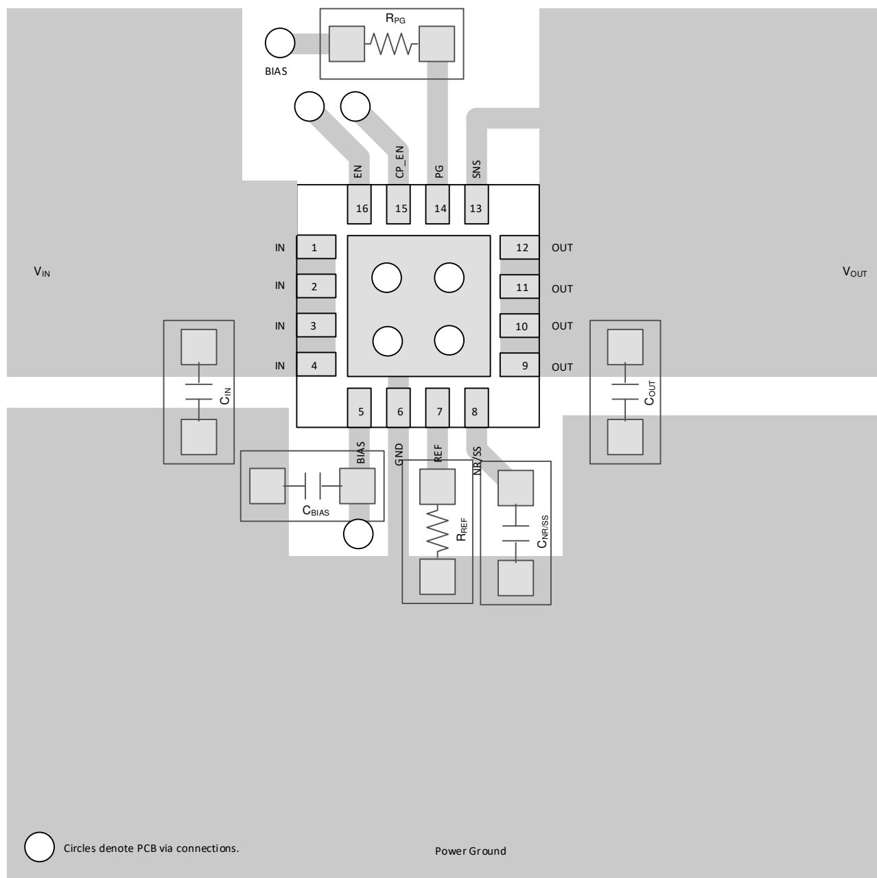
图 8-44. Recommended Layout
