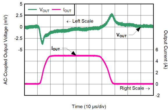
图 6-47. Load Transient for V_{OUT} = 5.2\text{ V} , I_{OUT} = 100\text{ mA} to 5\text{ A} , CP Disabled, SR = 1\text{ A}/\mu\text{s} , V_{BIAS} = 11\text{ V}
