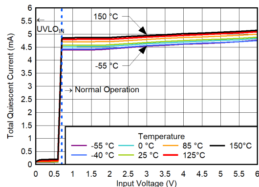
图 6-150. Total Pin Quiescent Current vs V_{IN} for V_{OUT} = 0.5\text{ V} , V_{BIAS} = 3.7\text{ V} , CP Disabled
