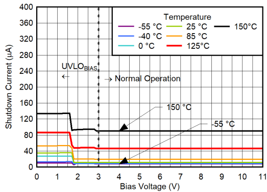
图 6-201. Total Shutdown Current vs V_{BIAS} for V_{IN} = 6\text{ V} , V_{OUT(nom)} = 0.5\text{ V} , CP Enabled
