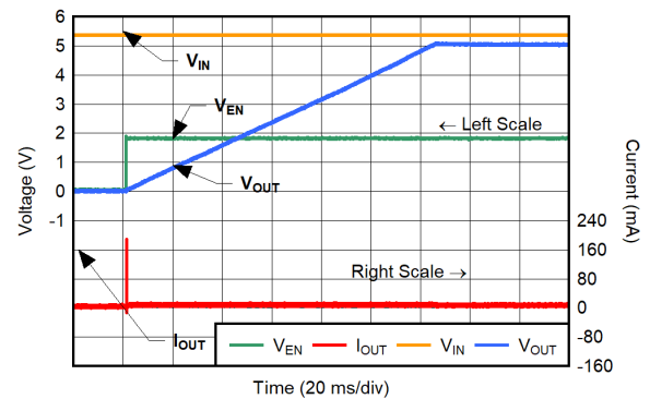
图 6-64. Inrush Current for CP Disabled, V_{OUT} = 5.2\text{ V}
