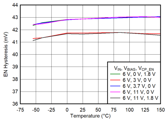
图 6-211. EN Hysteresis vs Temperature for V_{IN} = 6\text{ V} , V_{OUT} = 0.5\text{ V}
