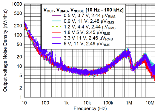
图 6-31. Output Voltage Noise Density vs Frequency and V_{OUT} for CP Disabled
