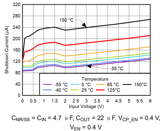
图 6-192. Total Shutdown Current vs V_{IN} for V_{OUT} = 0.5\text{ V} , V_{BIAS} = 11\text{ V} , CP Disabled
