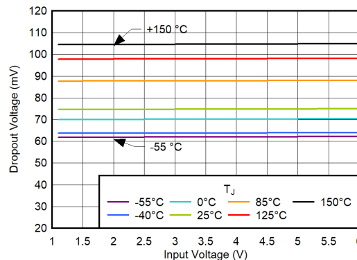
图 6-66. Dropout Voltage vs V_{IN} for CP Enabled, No Bias Rail
