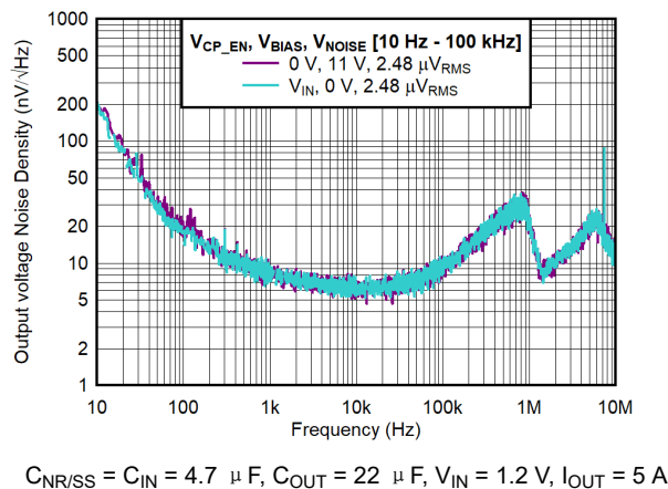
图 6-21. Output Voltage Noise Density vs Frequency and V_{CP\_EN} for V_{OUT} = 0.9\text{ V}
