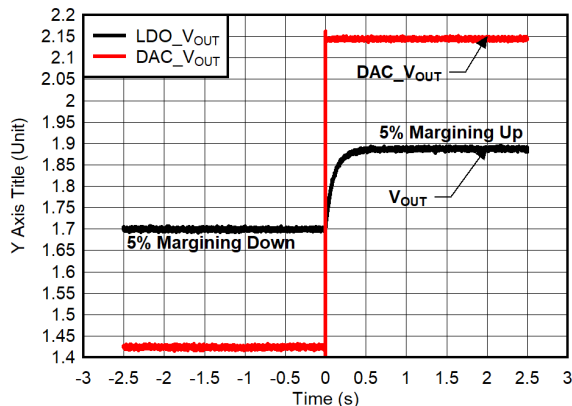
图 8-27. Margining From -5% to +5%
