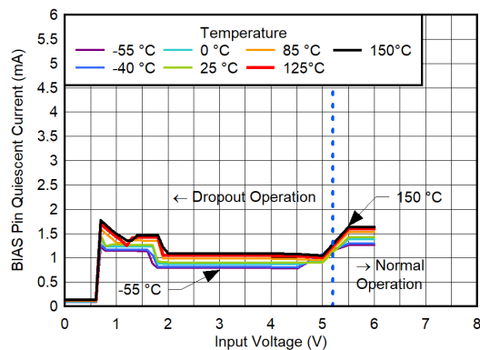
图 6-138. BIAS Pin Quiescent Current vs V_{IN} for V_{OUT} = 5.2\text{ V} , V_{BIAS} = 8.4\text{ V} , CP Disabled
