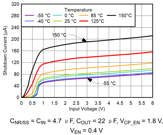
图 6-189. Shutdown Current vs V_{IN} for V_{OUT} = 0.5\text{ V} , V_{BIAS} = 0\text{ V} , CP Enabled
