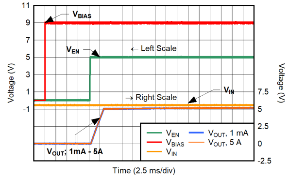
图 6-60. Start-Up for IN-BIAS-EN Rail Sequence for CP Disabled, V_{OUT} = 5.2\text{ V} , C_{NR/SS} = 100\text{ nF}
