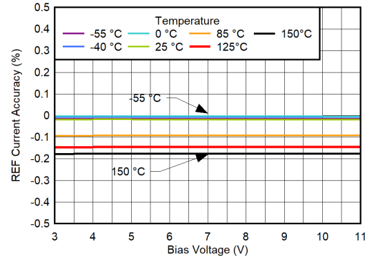
图 6-88. Reference Current Accuracy vs V_{BIAS} for CP Enabled, I_{OUT} = 0\text{ A}
