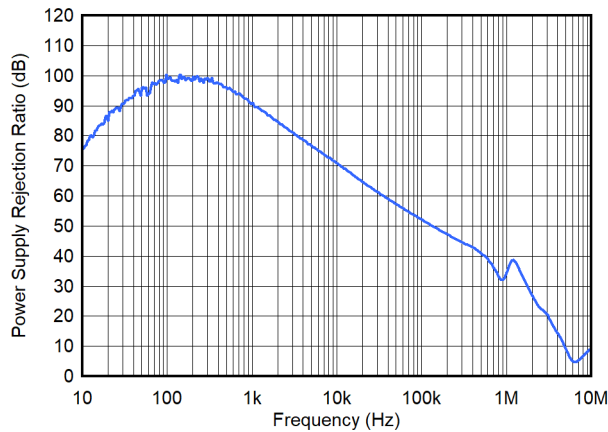
图 8-40. PSRR vs Frequency
