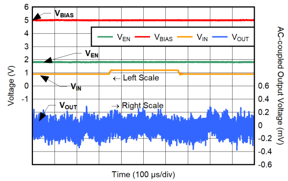
图 6-48. IN Line Transient for V_{IN} = 0.9\text{ V} to 1.2\text{ V}
