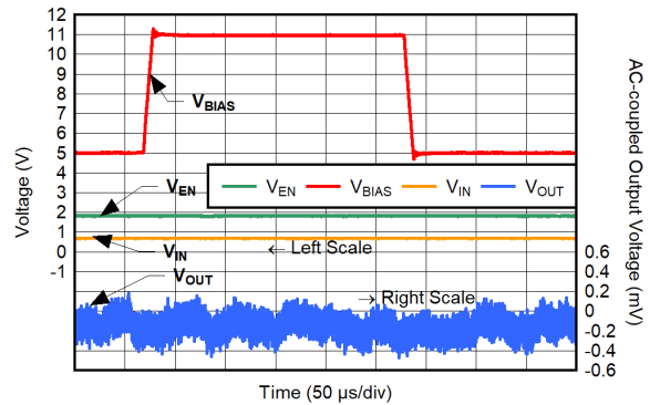
图 6-50. BIAS Line Transient for V_{IN} = 0.9\text{ V} to 6\text{ V} , I_{OUT} = 100\text{ mA}
