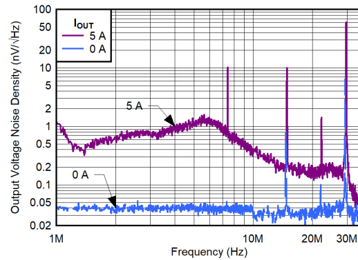
图 6-32. Charge Pump Output Voltage Noise Density vs Frequency and I_{OUT}
