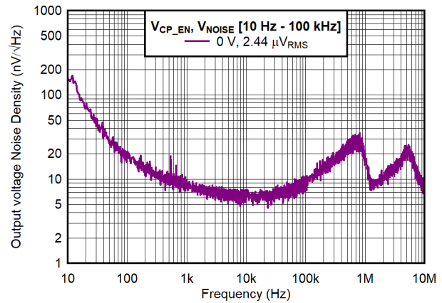
图 8-41. Noise vs Frequency
