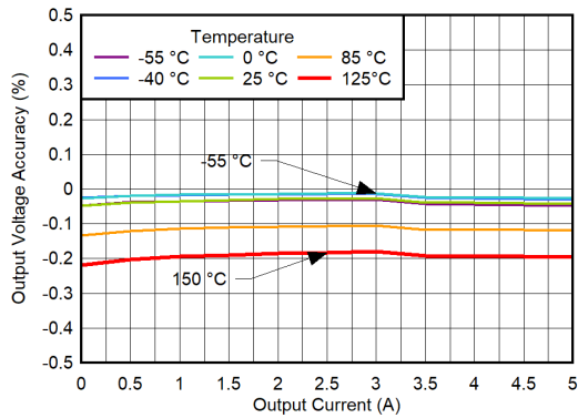
图 6-117. Output Voltage Accuracy vs I_{OUT} for V_{IN} = 5.6\text{ V} , V_{BIAS} = 11\text{ V} , CP Enabled
