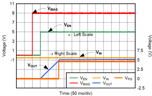
图 6-59. Start-Up for IN-CP_EN-EN Rail Sequence for CP Enabled
