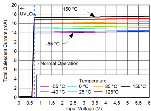
图 6-157. Total Quiescent Current vs V_{IN} for V_{OUT} = 0.5\text{ V} , V_{BIAS} = 3\text{ V} , CP Enabled, I_{OUT} = 0\text{ A}
