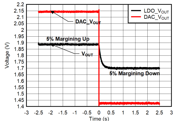
图 8-28. Margining from +5% to -5%
