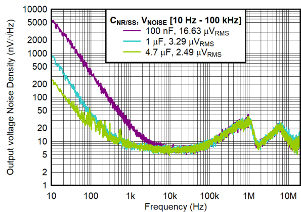
图 8-7. Output Voltage Noise Density vs C_{NR/SS} With Charge Pump Disabled
