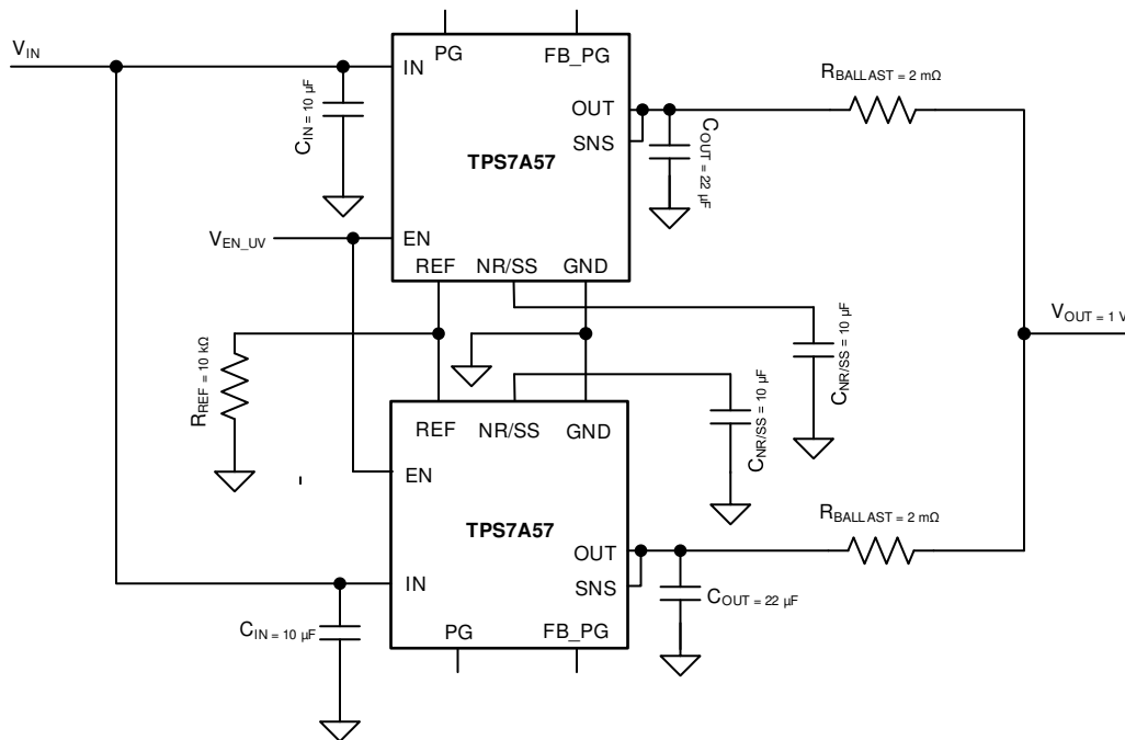
图 8-22. Paralleling Multiple TPS7A57 Devices
