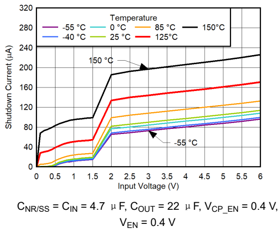
图 6-191. IN Pin Shutdown Current vs V_{IN} for V_{OUT} = 0.5\text{ V} , V_{BIAS} = 11\text{ V} , CP Disabled
