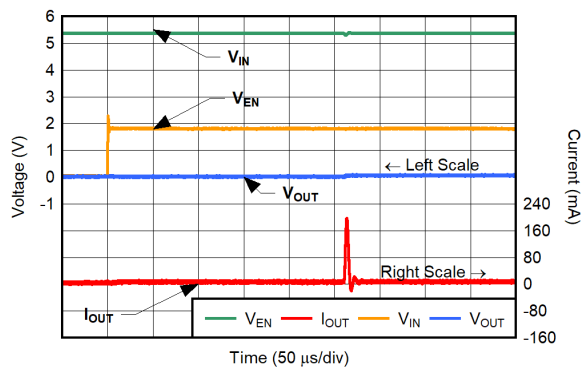
图 6-65. Inrush Current for CP Disabled, V_{OUT} = 5.2\text{ V} , First 500\text{ }\mu\text{s}
