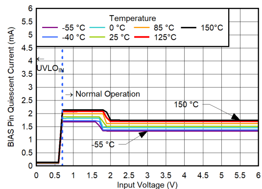
图 6-146. BIAS Pin Current vs V_{IN} for V_{OUT} = 0.5 \text{ V} , V_{BIAS} = 11 \text{ V} , CP Disabled
