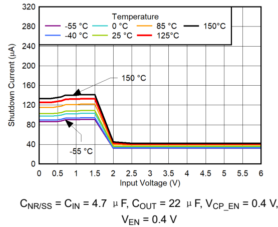
图 6-190. BIAS Pin Shutdown Current vs V_{IN} for V_{OUT} = 0.5\text{ V} , V_{BIAS} = 11\text{ V} , CP Disabled
