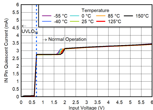
图 6-148. IN Pin Quiescent Current vs V_{IN} for V_{OUT} = 0.5\text{ V} , V_{BIAS} = 11\text{ V} , CP Disabled
