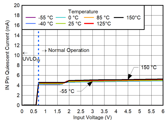
图 6-158. IN Pin Quiescent Current vs V_{IN} for V_{OUT} = 0.5\text{ V} , V_{BIAS} = 3\text{ V} , CP Enabled, I_{OUT} = 0\text{ A}
