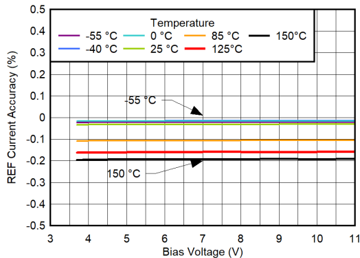
图 6-87. Reference Current Accuracy vs V_{BIAS} for CP Disabled, I_{OUT} = 0\text{ A}
