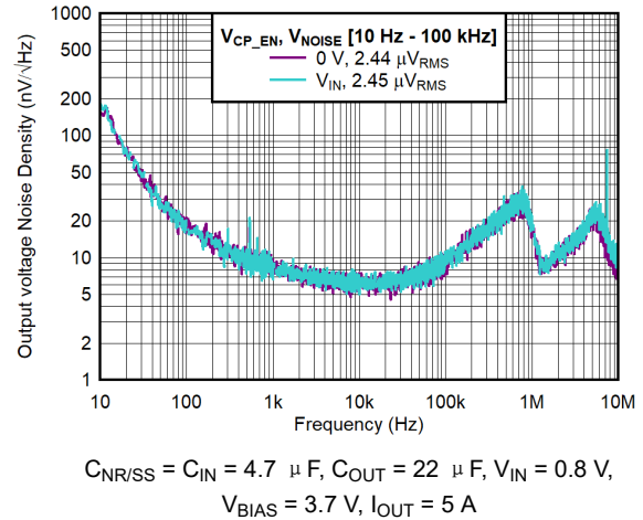
图 6-20. Output Voltage Noise Density vs Frequency and V_{CP\_EN} for V_{OUT} = 0.5\text{ V}
