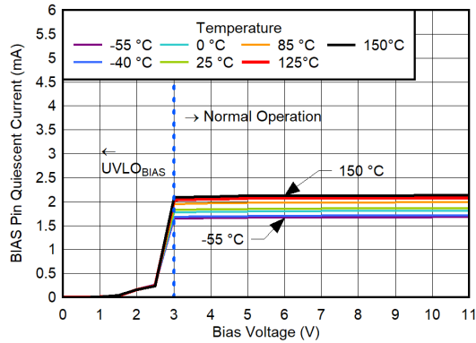
图 6-177. BIAS Pin Quiescent Current vs V_{BIAS} for V_{OUT} = 0.5\text{ V} , V_{IN} = 0.7\text{ V} , CP Disabled, I_{OUT} = 0\text{ A}
