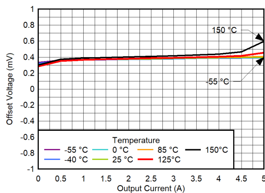
图 6-92. Offset Voltage vs I_{OUT}
