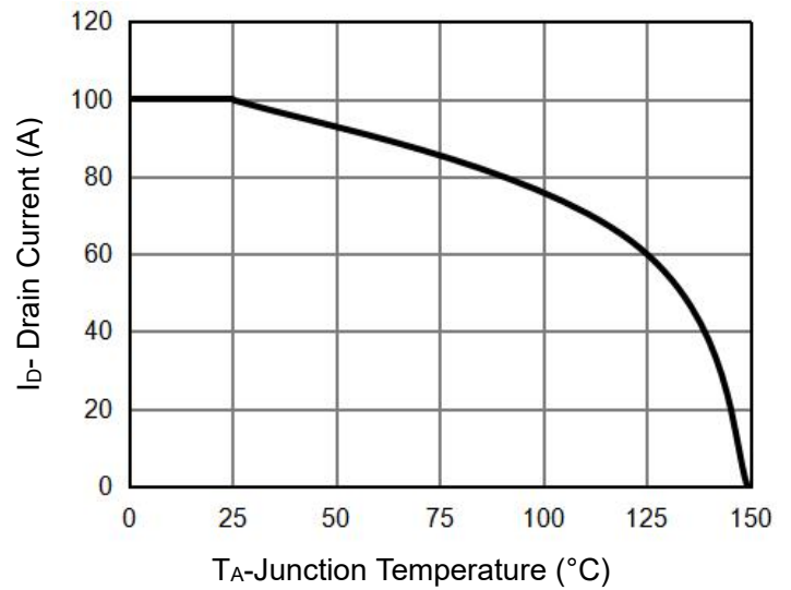
Figure 10 Current De-rating
