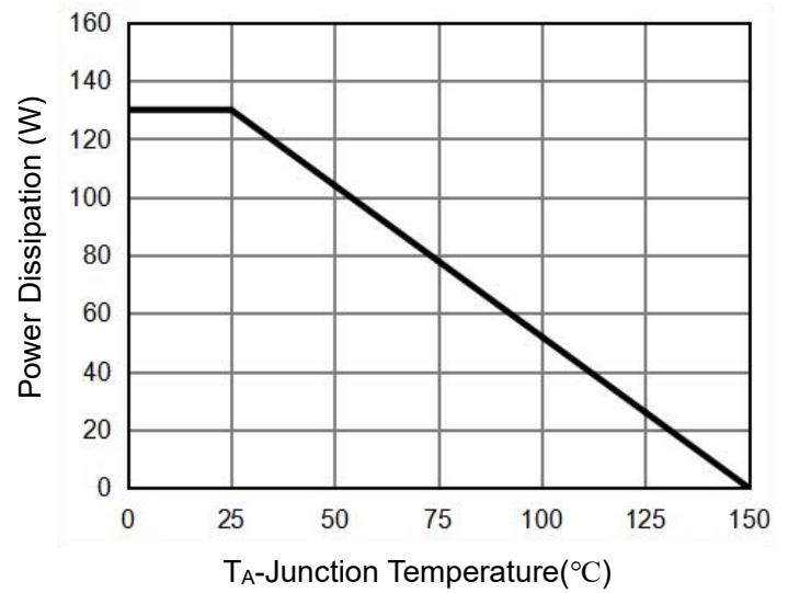
Figure 9 Power De-rating
