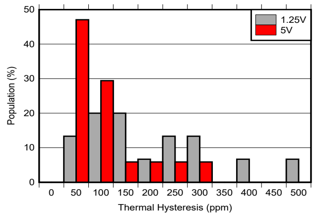
Figure 6-24. Thermal Hysteresis Histogram -40^\circ\text{C} to 125^\circ\text{C} Cycle 1
