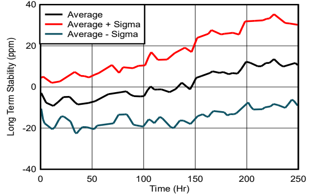
Figure 6-22. Long-Term Stability: 0 to 250 Hours
