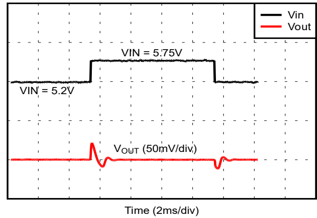
Figure 6-20. Line Transient Response
