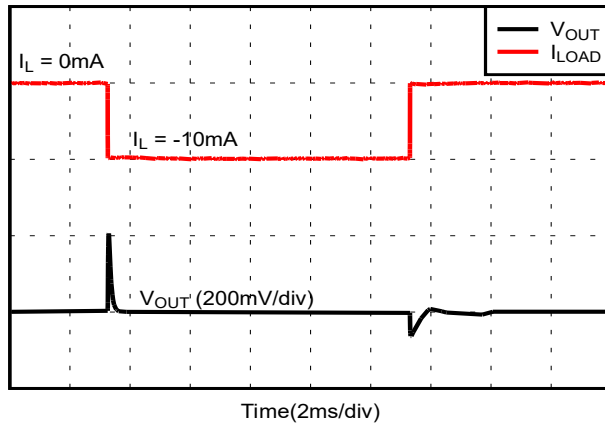
Figure 6-19. Load Transient Response (Sinking Current)
