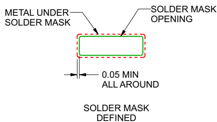
SOLDER MASK DETAILS NOT TO SCALE
