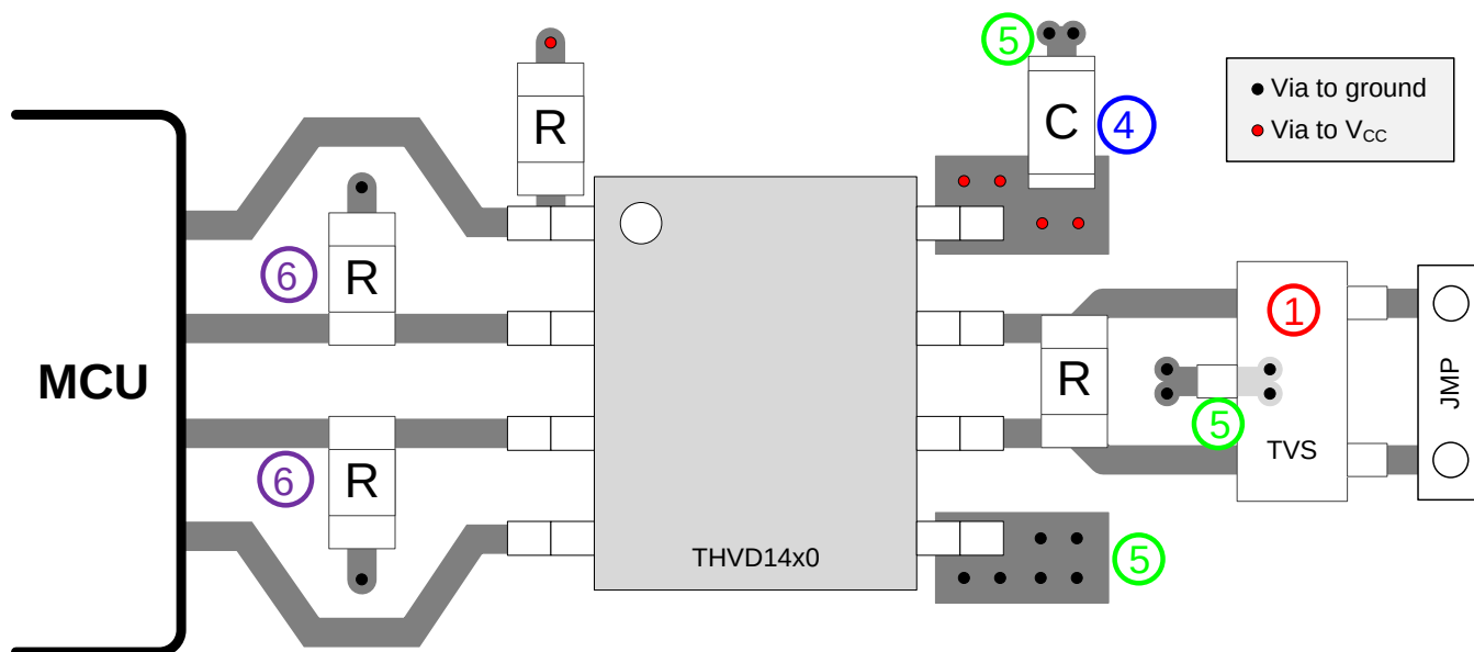
图 40. Half-Duplex Layout Example
